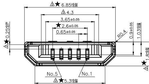
DETAIL A (2:1)
