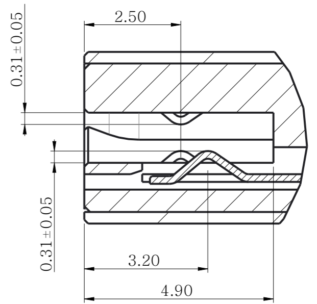
DETAIL A SCALE 10/1
