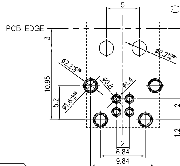
RECOMMENDED PCB LAYOUT (t=1.6)
