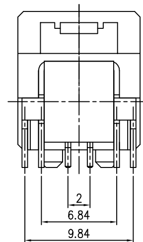
RECOMMENDED PCB LAYOUT (t=1.6)
