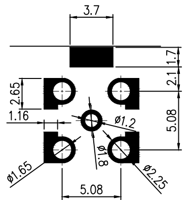
PCB LAYOUT (General Tolerance: \pm 0.05 )
