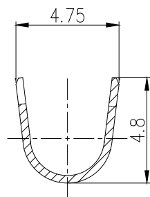
Section C-C' (Scale 4:1)
