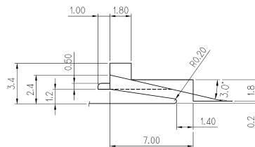
DETAIL LANCE (S=5/1)
