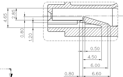
DETAIL 'C, (4/1)
