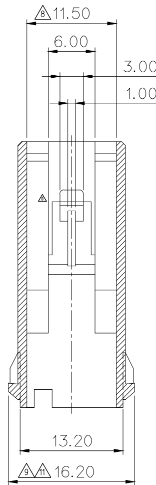
SECTION. B-B
