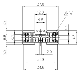
DETAIL 'A'(S=5/1) (TM/L 삽입부 DIMENSION)
