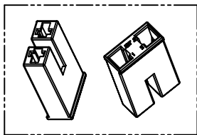
3D VIEW(참고용)
