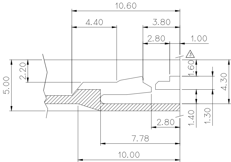
DETAIL B (5/1) (SECTION A-A)
