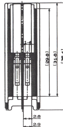
SEC. B-B
