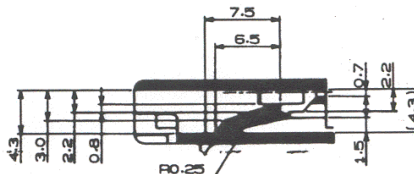
DETAIL. C
