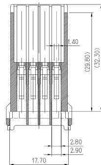
SEC. B-B
