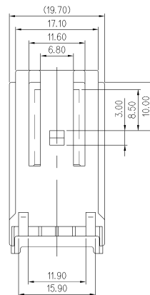
SEC. B-B
