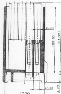
SEC. B-B
