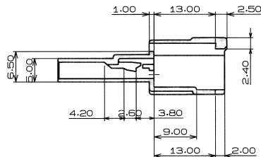
SEC. A - A
