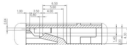
DETAIL 'B,(S:5/1)
