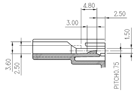
DETAIL LANCE(PAXS=2/1)
