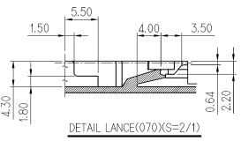
DETAIL LANCE(070)(XS=2/1)
