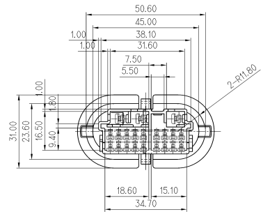
DETAIL LANCE(070)(XS=2/1)
