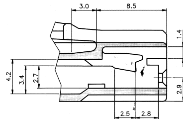
TERM* LOCK부 DETAIL (5/1)
