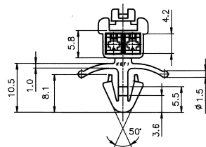
TERM* LOCK부 DETAIL (5/1)
