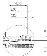
DETAIL 'B, (5/1)
