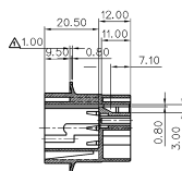
SEC. B-B
