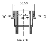
SEC. C-C
