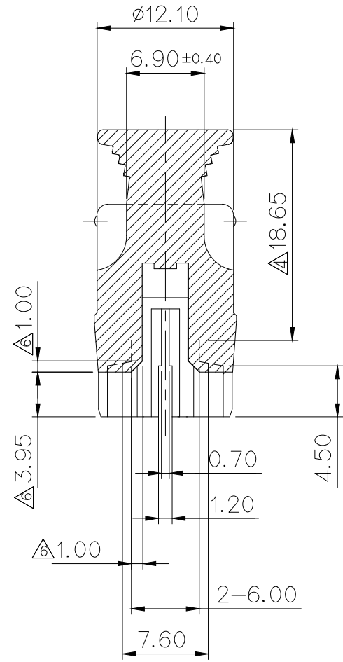
SECTION B-B
