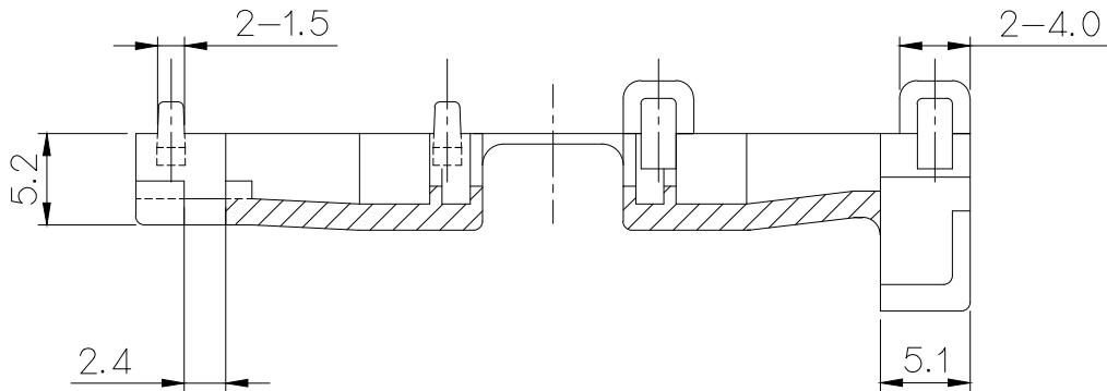
SECTION A-A(2/1)
