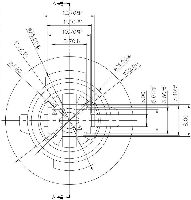
BULB ASS'Y(참고)
