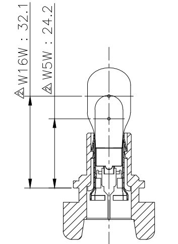
BULB ASS'Y(참고)
