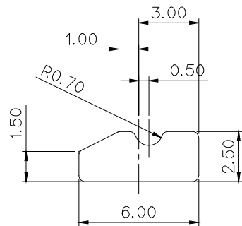
VIEW "W" (S= 5/1)
