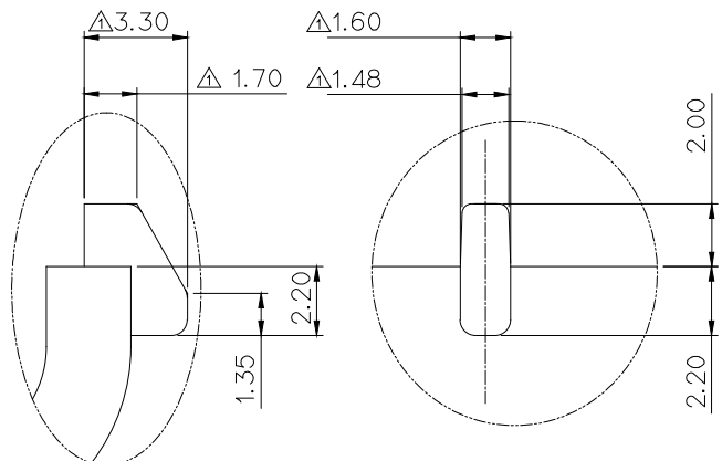
LOCK "E" SCALE 5/1
