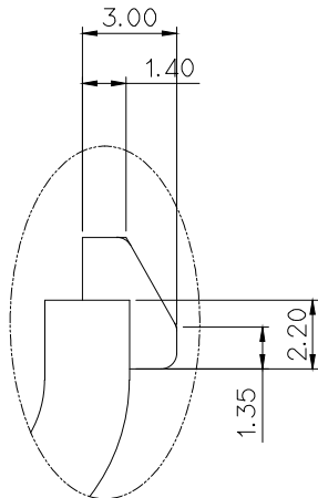
LOCK "C" SCALE 5/1
