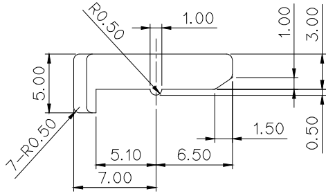
VIEW "W"(4:1)
