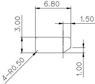
VIEW "X"(4:1)
