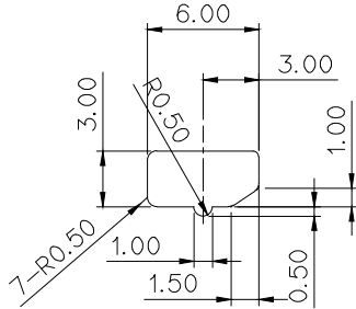
VIEW "Y"(4:1)
