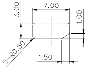
VIEW "Z"(4:1)
