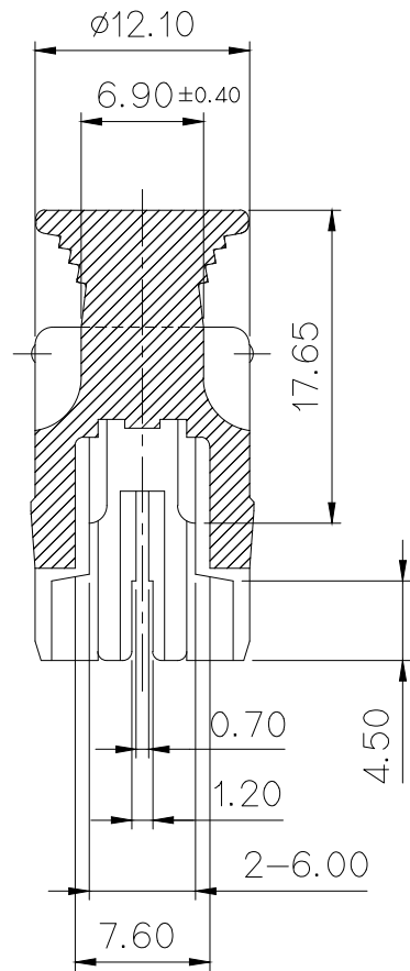
SECTION B-B
