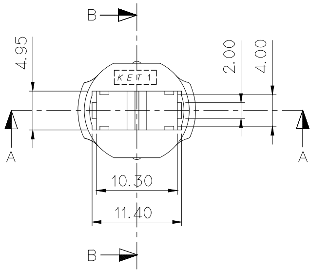
VIEW "C"
