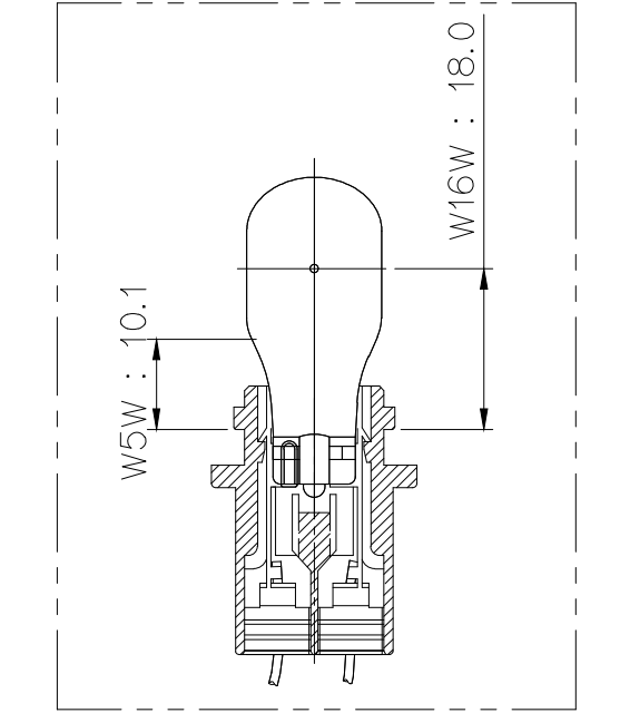
BULB HOLDER ASSY(S:1/1)
