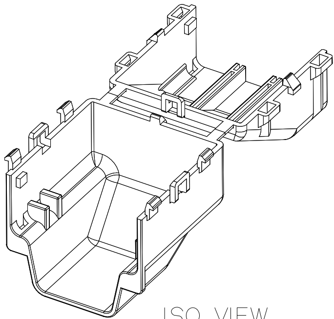
ISO VIEW
