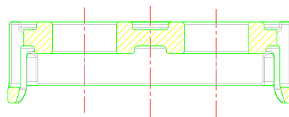
SECTION C-C
