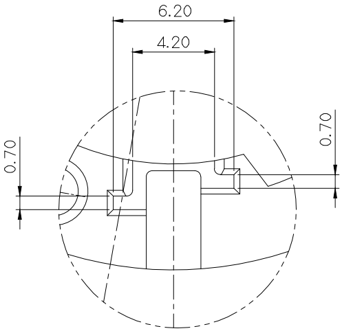
△ DETAIL Z (S=5/1)
