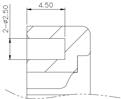
SECTION B-B(S=5/1)
