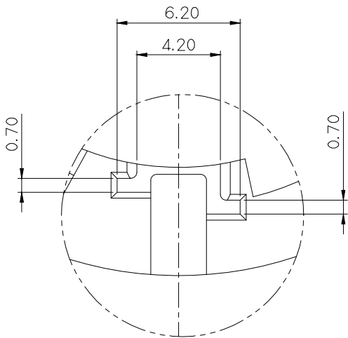
△ DETAIL Y (S=5/1)
