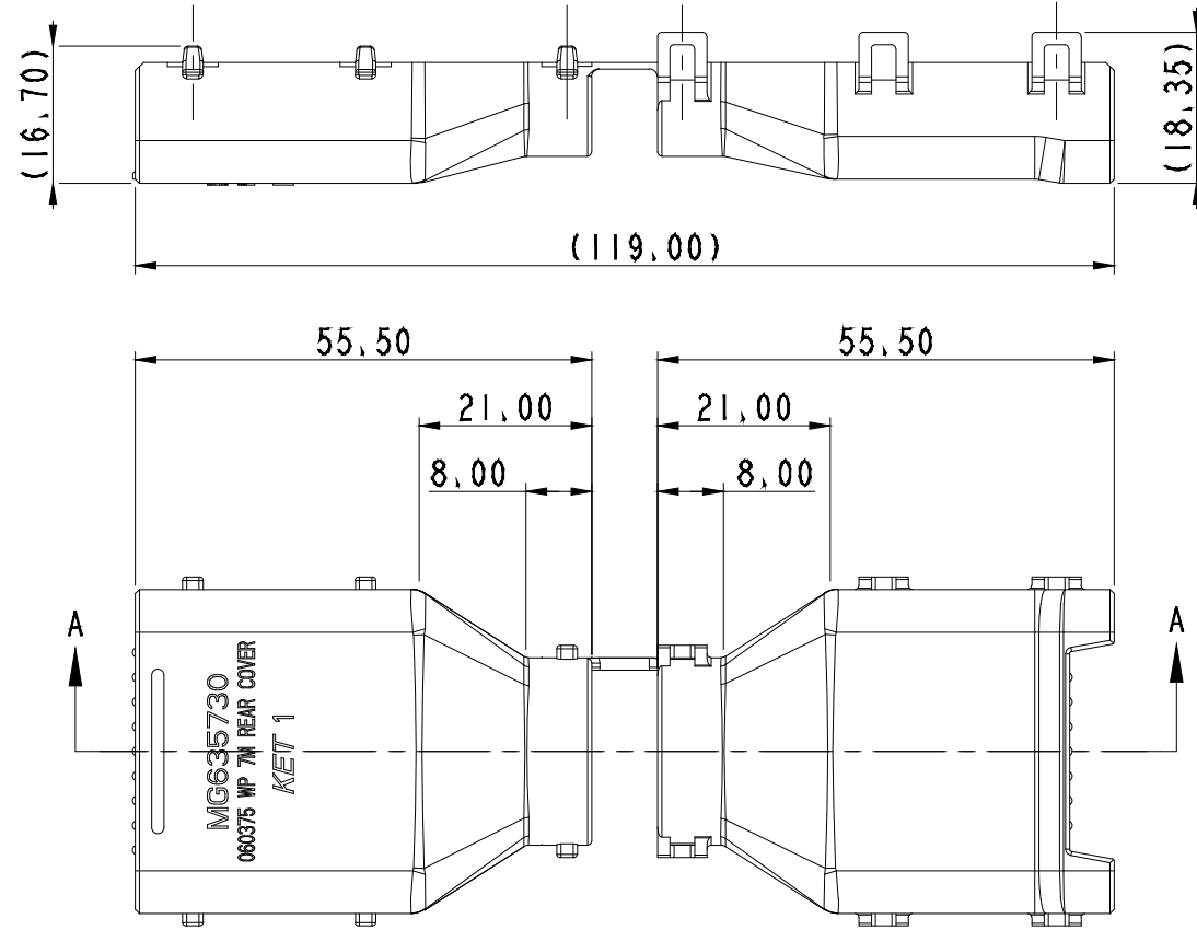
ISO VIEW SCALE 1/2
