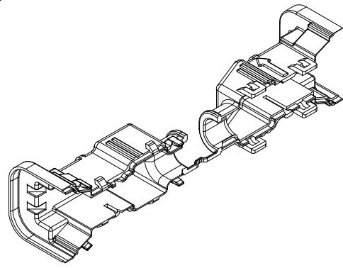
ISO VIEW
