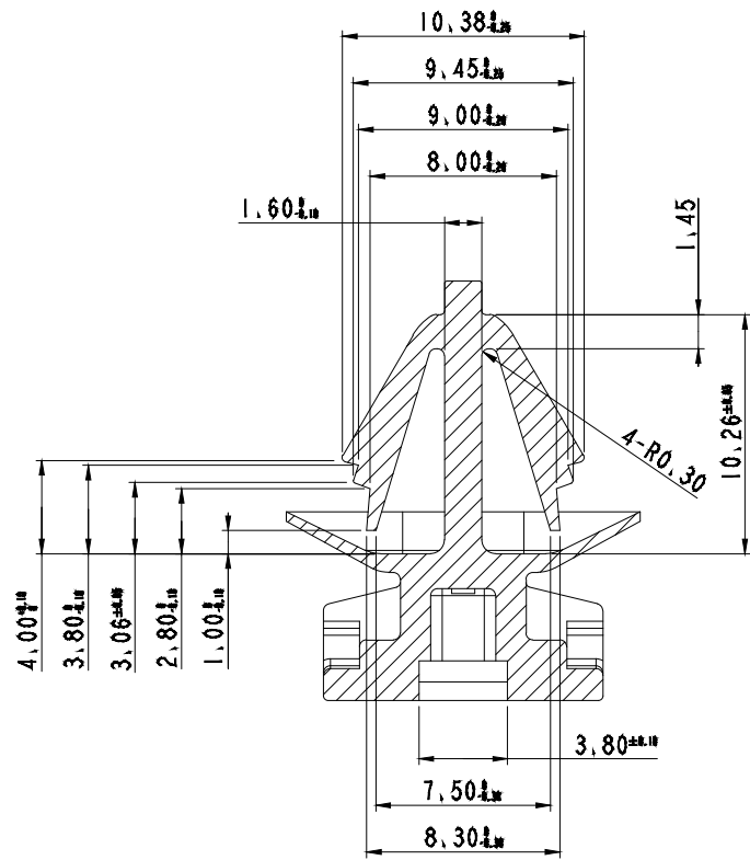
SECTION B-B SCALE 4/1
