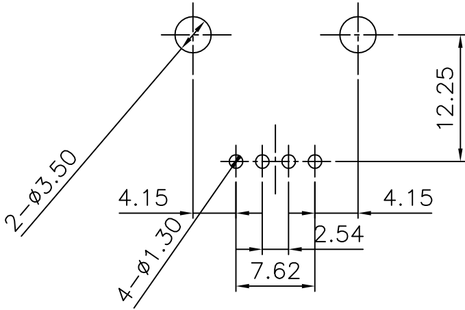
PRINT CIRCUIT BOARD PITCH (TLERANCE ±0.1)
