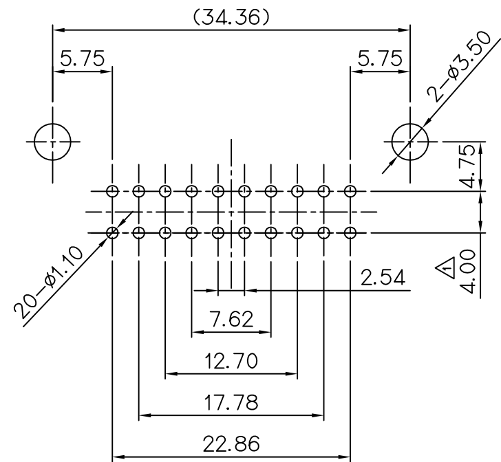
PRINT CIRCUIT BOARD PITCH (TOLERANCE ±0.1)
