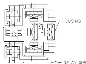
RELAY & HS'G ASS'Y SCALE 2:1
