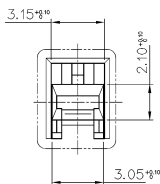
DETAIL B (S=5/1)
