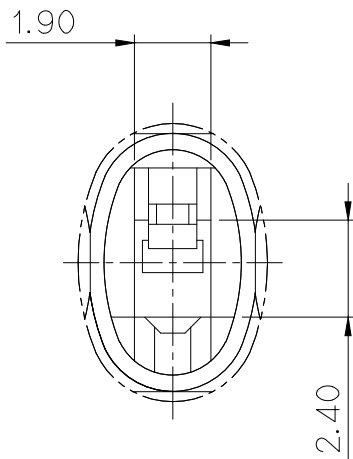
△△DETAIL B(S=5/1) (TERMINAL 삽입부 DIMENSION)
