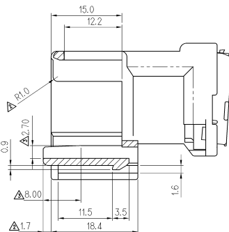
SECT. A-A
