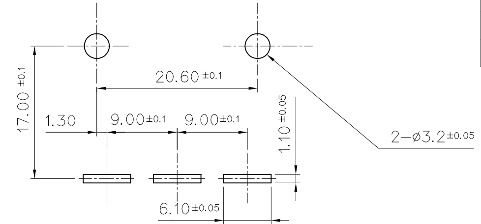
PCB BOARD LAYOUT (t=1.6mm)
