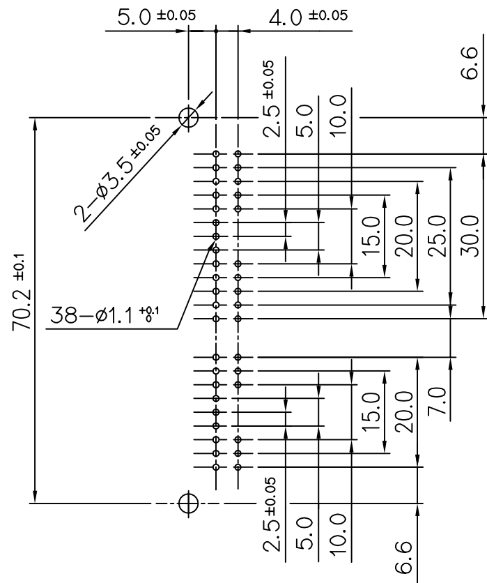
PRINT CIRCUIT BOARD LAYOUT(t=1.6mm) (TOLERANCE : ±0.1)
