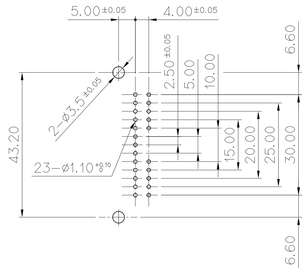
PRINT CIRCUIT BOARD LAYOUT(t=1.6mm) (TOLERANCE : ±0.10)
