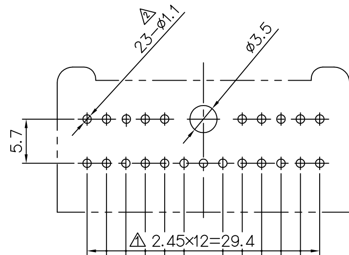
PRINT CRCUIT BOARD LAYOUT(t=1.6mm) TOLERANCE: ±0.10(SCALE:2/1)
