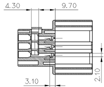
SECTION B-B ( 090 )
