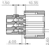
SECTION C-C ( 187 )
