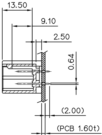
SEC. B-B
