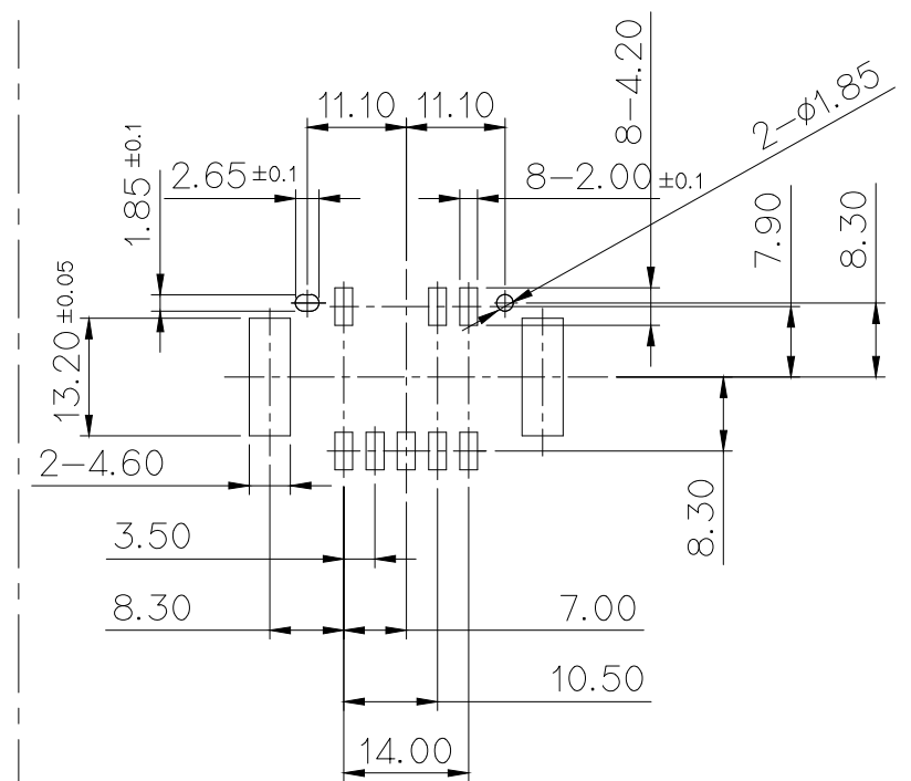
P.C.B. LAYOUT(S=1/1) (GENERAL TOLERANCE : ±0.1)
