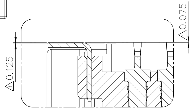
△DETAIL "Z" (S=4/1)
