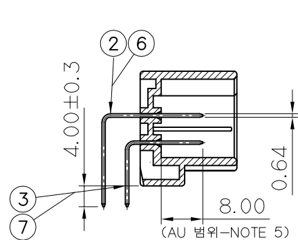
SECTION B-B (070II SECTION)
