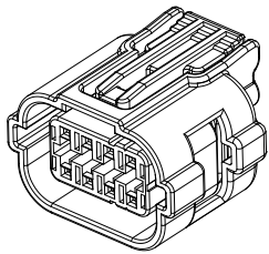
ISO VIEW
