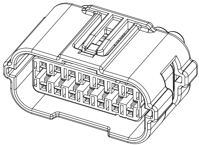
ISO VIEW
